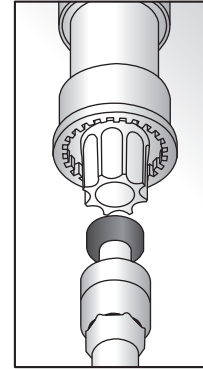
Shimano® Octalink & ISIS Drive®
